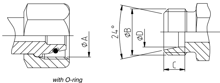
with O-ring
